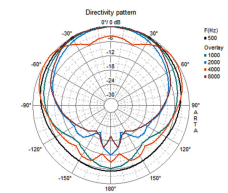
ESP-250WS Directivity horizontal
